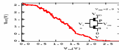
Figure 2-*First single nanotube logic device – Inverter demonstration. (Appl. Phys. Lett., Nov. 2001)
