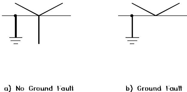
Fig.5: Voltage Profiles for Solidly Grounded System
