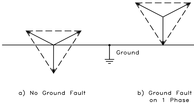
Fig.3 Voltages During Ground Fault
