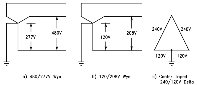
FIG. 6 Solidly Grounded Systems (Industrial/Commercial)
