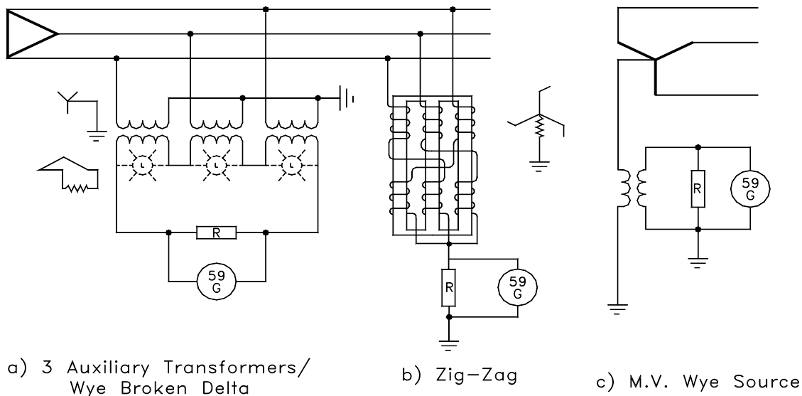
Fig.11 Grounding Transformers
