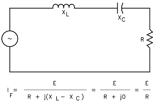
Fig. 7 Series Resonant Circuit (when X_L=X_C )
