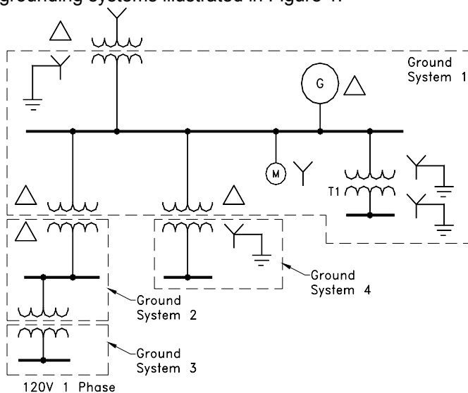
Fig.1 Grounding Systems
