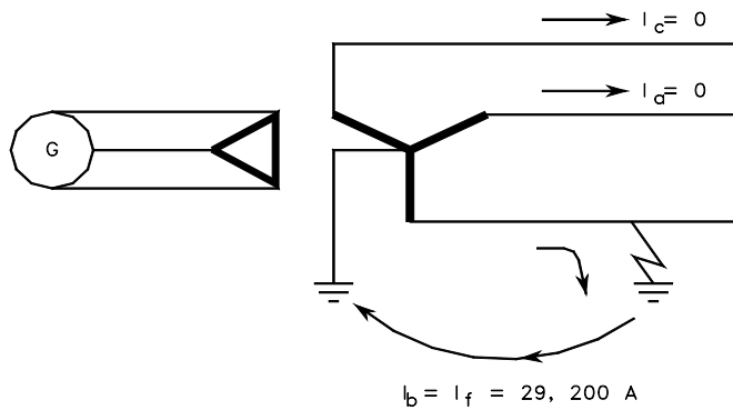
Fig.4: Ground Fault on a Solidly Grounded System
