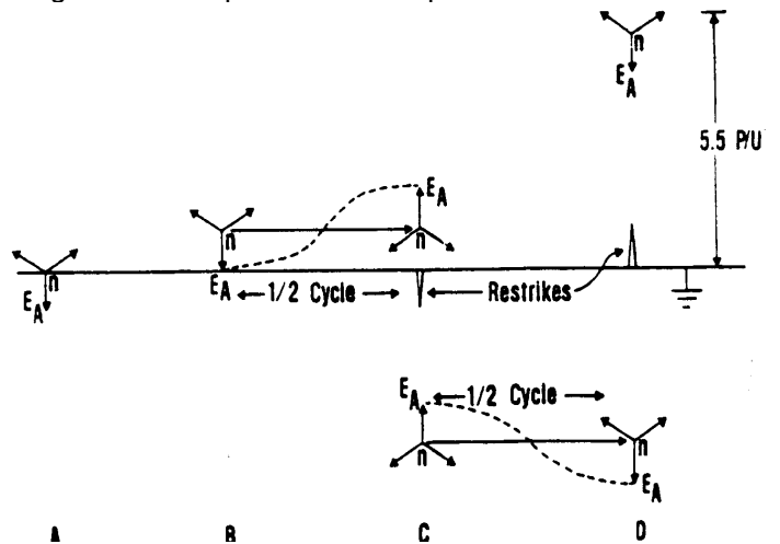
Fig.8 Transient Overvoltages from Restriking Ground Fault
