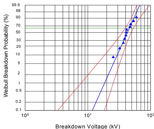
Fig. 1. Weibull distribution of 60 Hz breakdown voltages 11 cables \alpha = 45.9 kV peak \beta = 5.08 Confidence Intervals 95%
