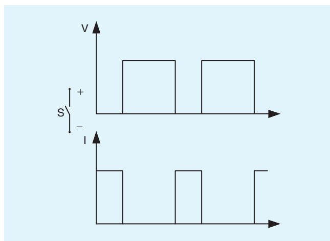
Fig. 3. Voltage and current waveforms in an ideal switch.
