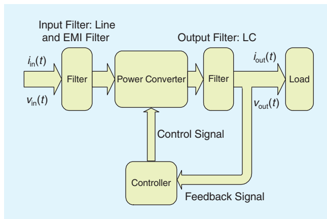
Fig. 1. A block diagram of a power electronic system.
