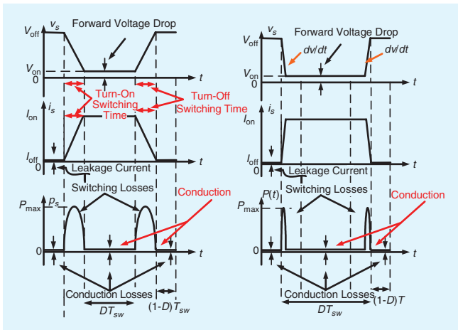
Fig. 6. Voltage, current and power waveforms of a switch at two different switching times.
