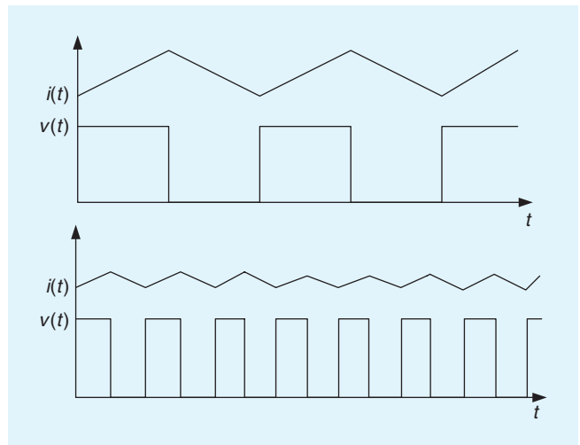
Fig. 7. Voltage and current waveforms at two different switching frequencies.
