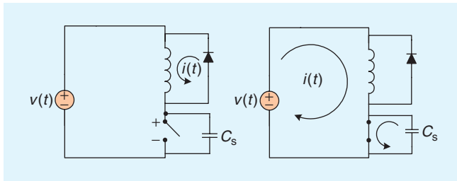
Fig. 5. Stray capacitance in a power converter and transient effect.
