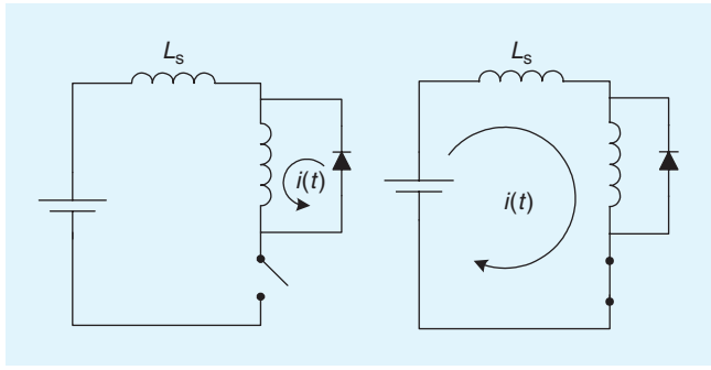
Fig. 4. Stray inductance of a current loop and transient effect.
