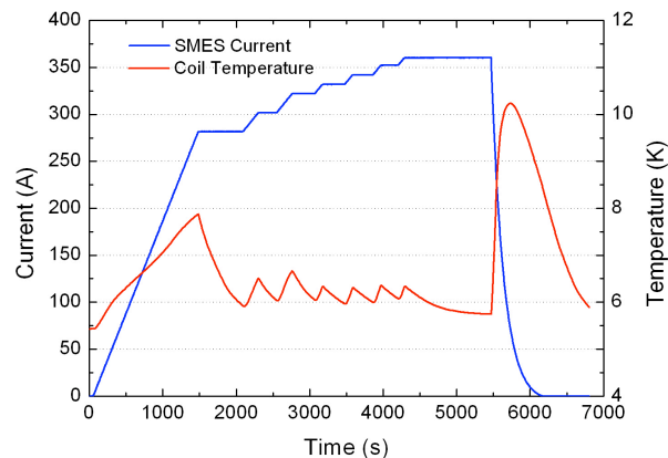
Fig. 1. Charge and discharge test results
