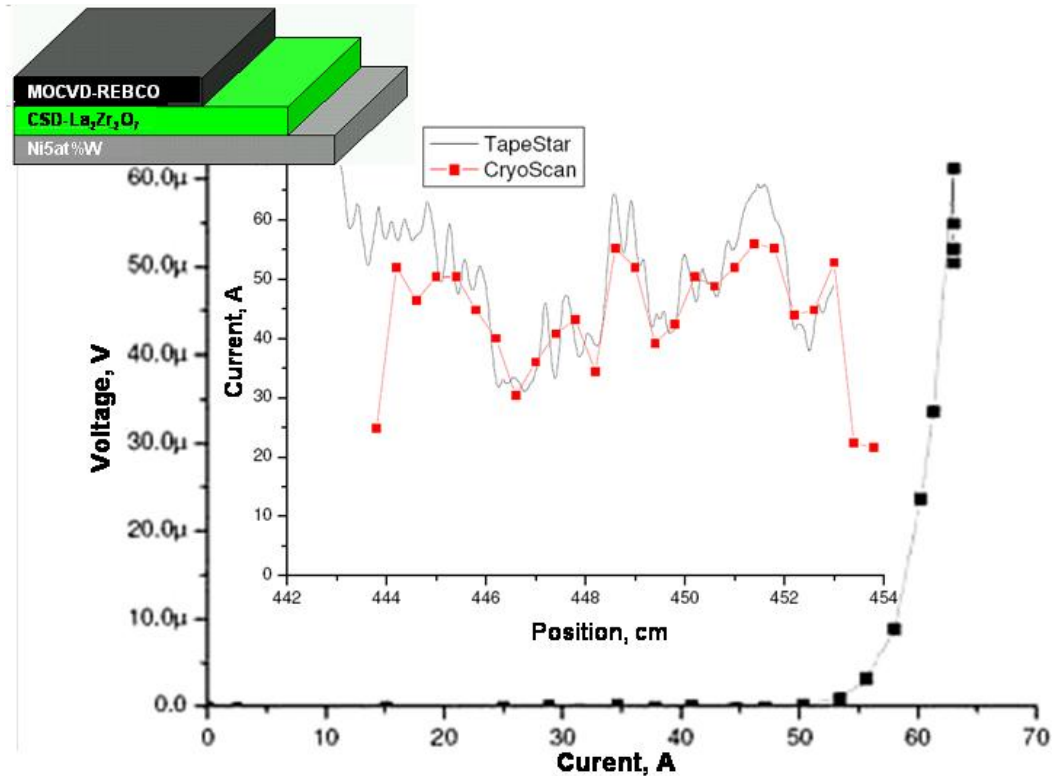
Fig. 3. Direct current measurements of MOCVD-YBCO/CSD-LZO/NiW. End-to-end critical current was measured as 57.9\pm 0.28 A/cm-width (0.1 m piece of a 4.4 m long tape, which had an end-to-end critical current of 21.0\pm 0.2 A). The inductively measured I_c value is shown in the inset. The CSD-buffer was produced by Nexans Superconductors and the critical currents were measured at THEVA by “TapeStar” and “CryoScan” [3] apparatus.
