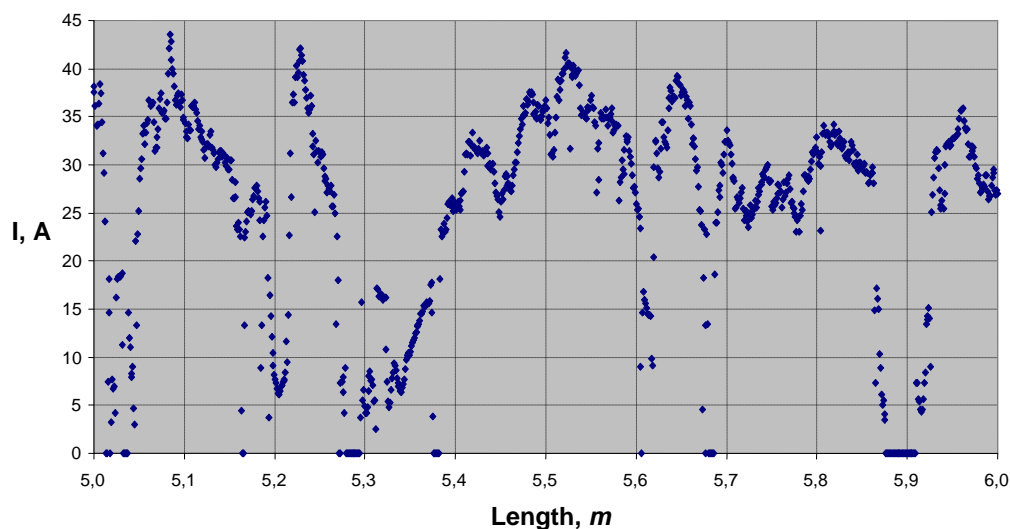
Fig. 2. Inductively measured I_c of a 1 m segment of a 10 m long all-MOCVD CC. The I_c over 'good' 0,1-0,2 m CC segments is 25-40 A. The YBCO thickness was \sim 350 nm, which corresponds to maximum current density j_c > 1 MA/cm 2 . The Tape Star (THEVA) measurement was performed at Zenergy Power [2].
