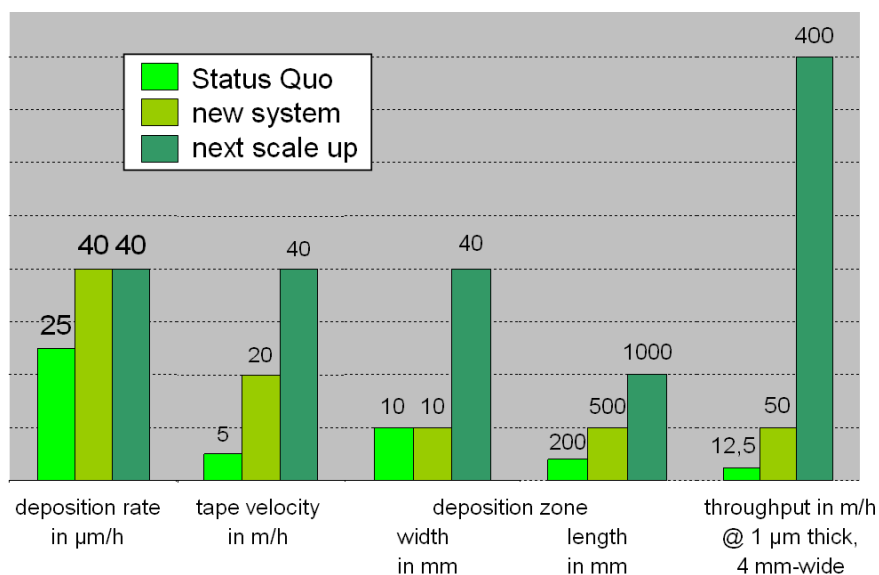
Fig. 5. Scale up plans for MOCVD of YBCO (Braunschweig activities only).
