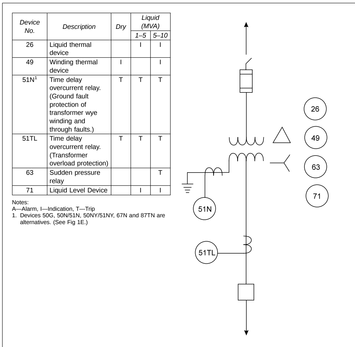
Fig. 1A. Electrical protection one-line. Primary fuse. 1000- to 10000-kVA transformers. Less than 1000 kVA when transformer creates fire exposure.
