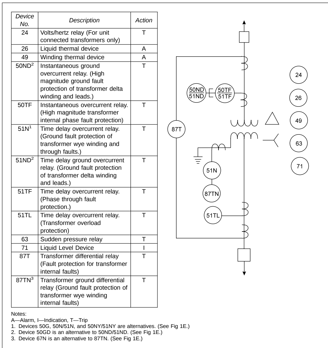
Fig. 1C. Electrical protection one-line. 10000-kVA and larger transformers.
