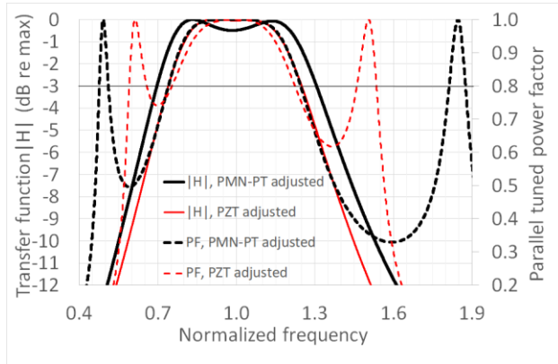
Fig. 3. Transfer function and parallel tuned power factor vs. normalized frequency for composites with one matching layer with conventional impedance Z_m=(Z_c Z_r)^{1/3} and adjusted thickness. Black, thick curves: PMN-28%PT composite, t=1.09\lambda/4 . Red, thin curves: PZT composite, t=1.07\lambda/4 .
