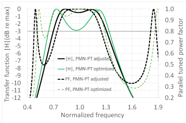
Fig. 4. Transfer function and parallel tuned power factor vs. normalized frequency for the PMN-28%PT composite with one matching layer. Black, thick curves: Conventional impedance Z_m=(Z_c Z_r)^{1/3} and adjusted thickness t=1.09\lambda/4 . Green, thin curves: Impedance and thickness optimized for maximum bandwidth, Z_m=1.4(Z_c Z_r)^{1/3} and adjusted thickness t=1.15\lambda/4 .
