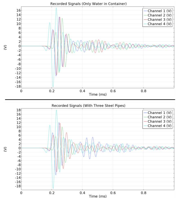
Fig. 3. Examples of recorded electric signals in two cases showed in Fig. 2.
