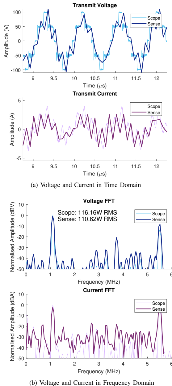
Fig. 4. HRPWM Output of GaN Pulser at 200 Vpp and 1.1 MHz into Sonic Concepts H-102 Transducer Measured By Keysight MSO-S 204A Oscilloscope an HIFUARP I-V Sense Circuitry.
