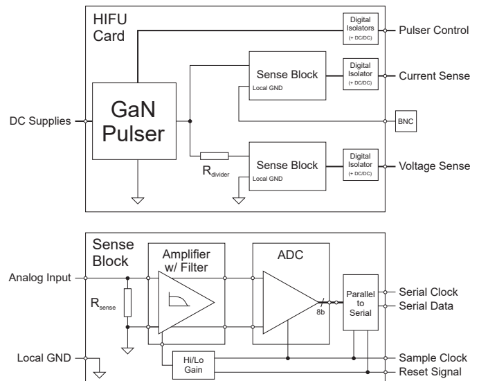
Fig. 1. Block Diagram of GaN Based HIFUARP Card with Current/Voltage Sense Circuitry.
