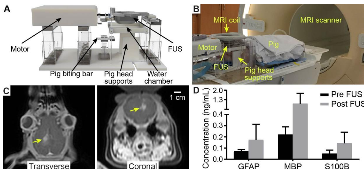
Fig. 1. A) 3D rendering of MR-compatible FUS-LBx system. B) Picture of experimental setup. C) Contrast-enhanced T1-weighted MR images verified successful BBB opening (yellow arrow). D) FUS-LBx enhanced the release of brain-specific biomarkers (GFAP, MBP, and S100B).
