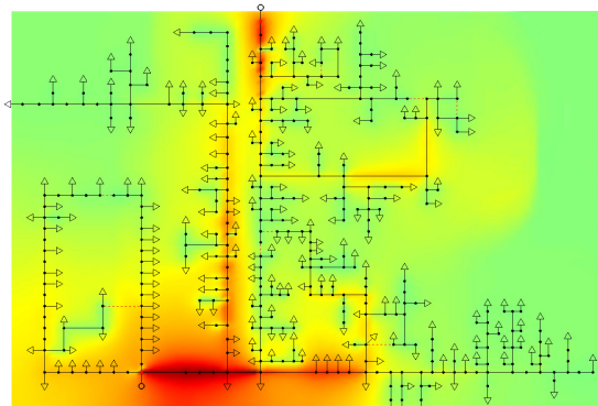
Fig. 10. Branches congestion levels for scenario 4 considering the dumb charging approach. Grading between light green and red, stand for increasing values of congestion, from 0 to 100%.
