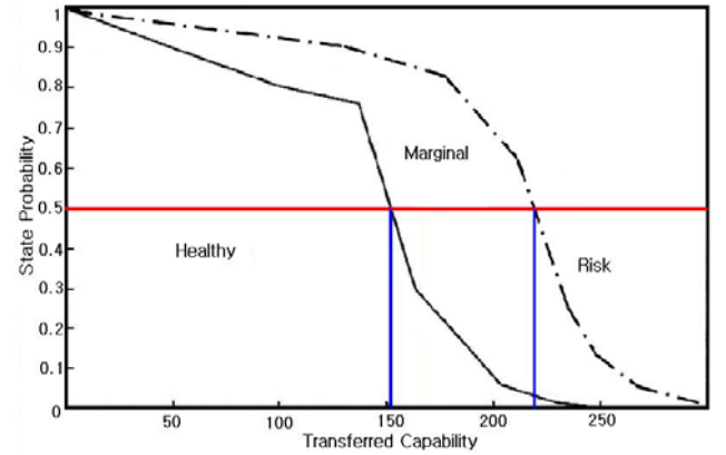
Fig 5. Computation of optimal capability using well-being method
