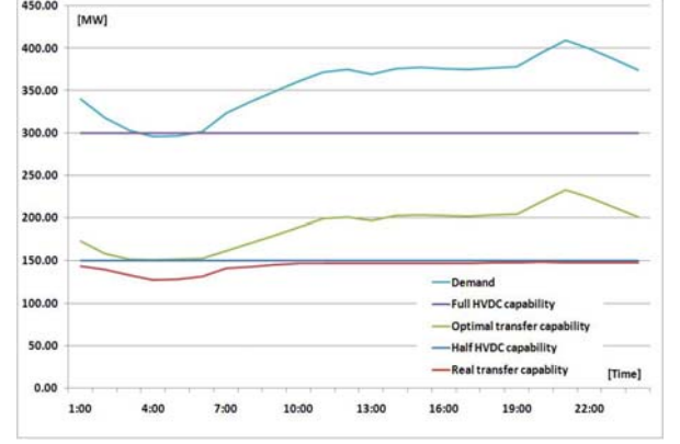
Fig 4. Computation of optimal capability using cost-optimization
