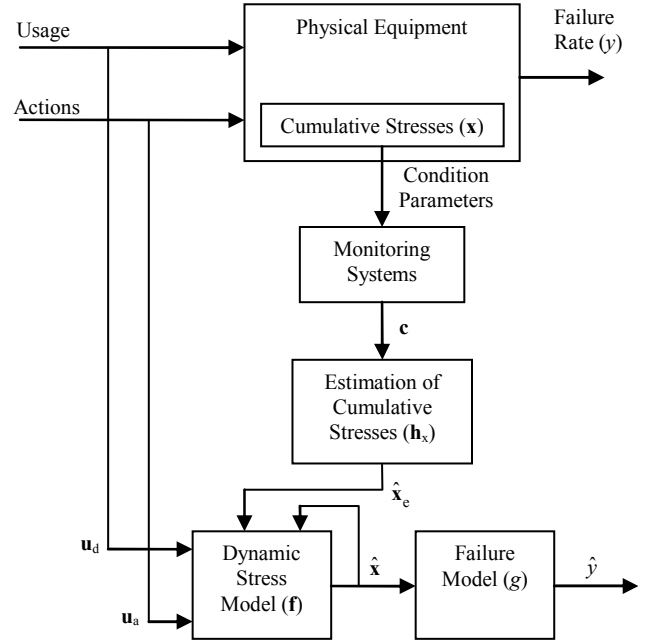
Fig. 1. Predictive Health Model.
