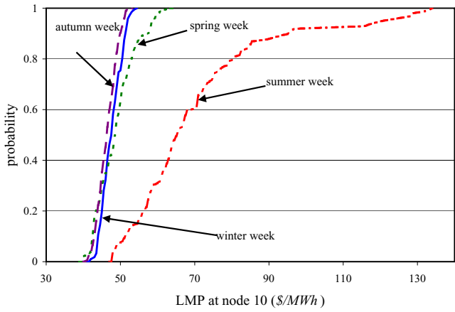
(a) c.d.f. of \underline{\Lambda}_{10}
