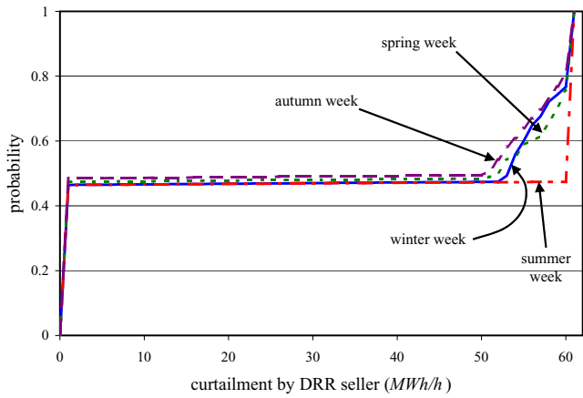
(b) c.d.f. of \hat{P}_r
