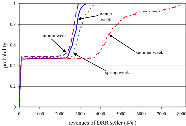
(c) c.d.f. of \underline{\Lambda}_{10} \cdot \hat{P}_r
