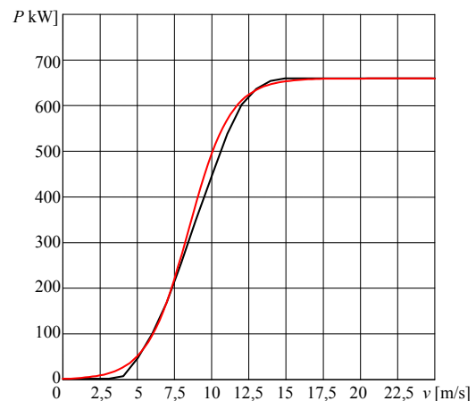
Fig. 1. Approximation of the power generated by a 660kW wind turbine through a sigmoid curve ( v_0=8,4686 ; w=-1,4 ); – measured curve; – approximated curve
