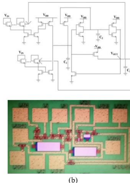
Fig. 2: Building blocks of NNIC: (a) synapse device and (b) neuron circuit
