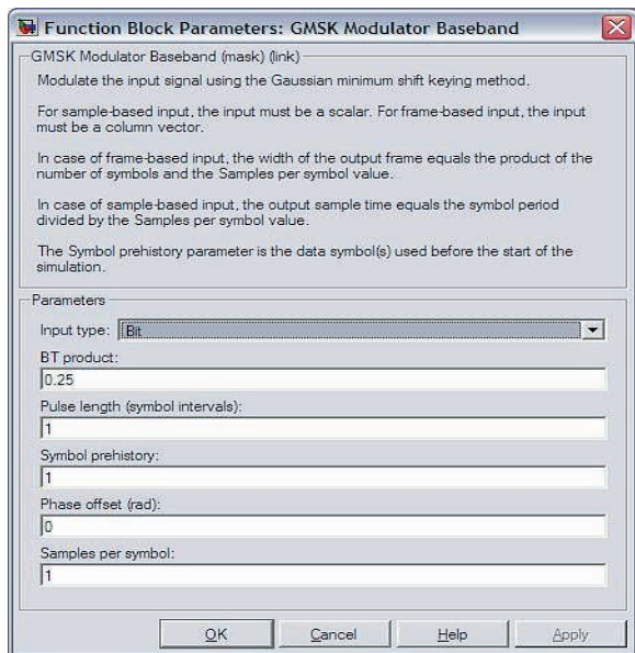
Figure 7: GMSK Block Mask
