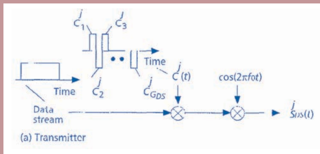
Figure 3: CDMA Block Diagram
