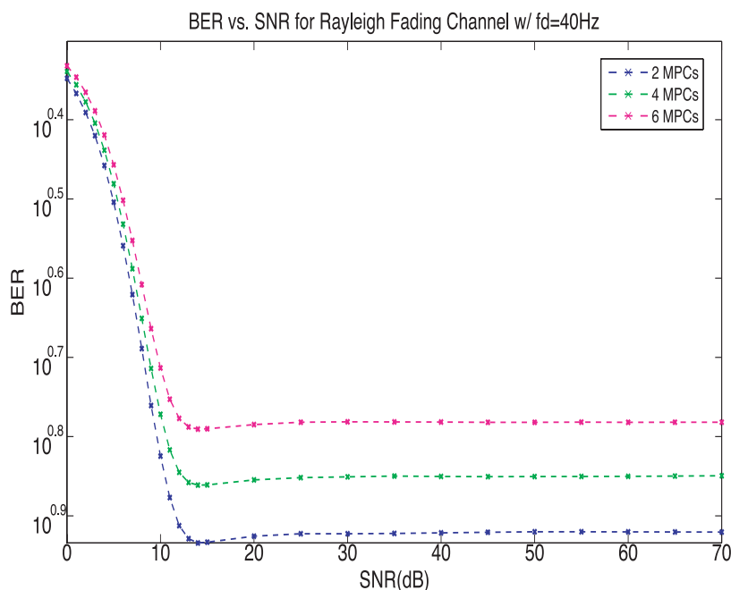
Figure 10: Performance under dynamic channel with fd=40Hz
