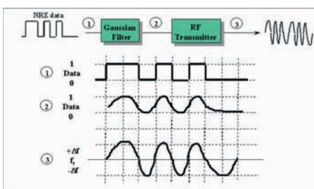
Figure 2: GMSK Block and Timing Diagrams (source: http://sna.csie.ndhu.edu.tw/~cnyang/mobile/sld083.htm )
