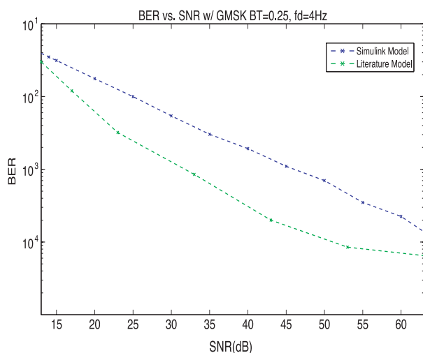
Figure 15: GMSK, BT=0.25, fd=4Hz
