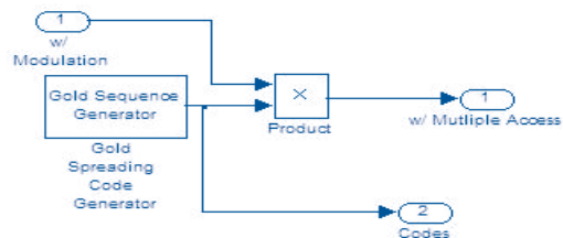
Figure 8: CDMA Block
