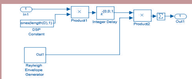
Figure 6: Multi-path Rayleigh Fading Block
