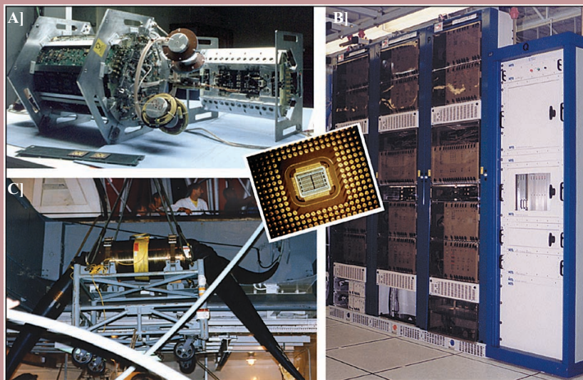
Figure 3: Scenes from the development of the Undersea Branching Multiplexers (UBMs): A] Engineering prototype of the UBM; B] Associated supervisory and terminal equipment C] The UBM aboard the ocean cable laying ship; INSERT: Application specific integrated circuit (ASIC) developed and qualified for the UBM.
