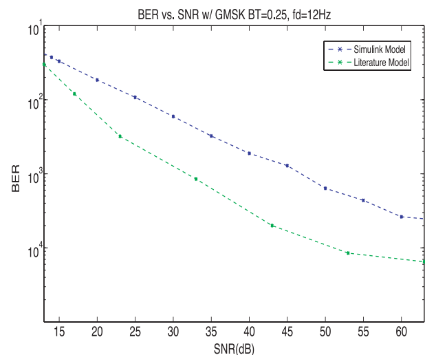
Figure 14: GMSK, BT=0.25 , f_d=12\text{Hz}
