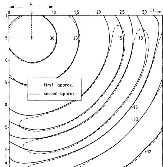
Fig. 2. Contour plot of the radiation pattern, after 141 time steps, of an isotropic source located at node (5, 5) of a 35*35-node mesh (arbitrary units).
