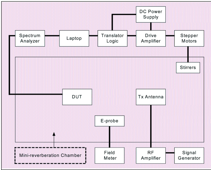
Figure 2. SE Measurement Set-up Employing Mini-reverberation Chamber Methodology.
