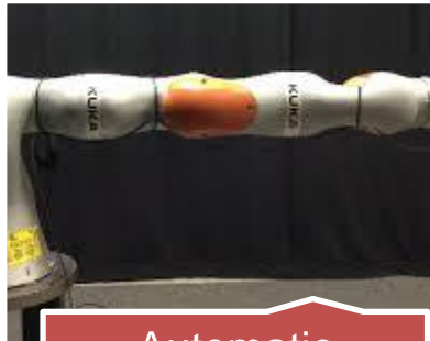
Collision Detection
