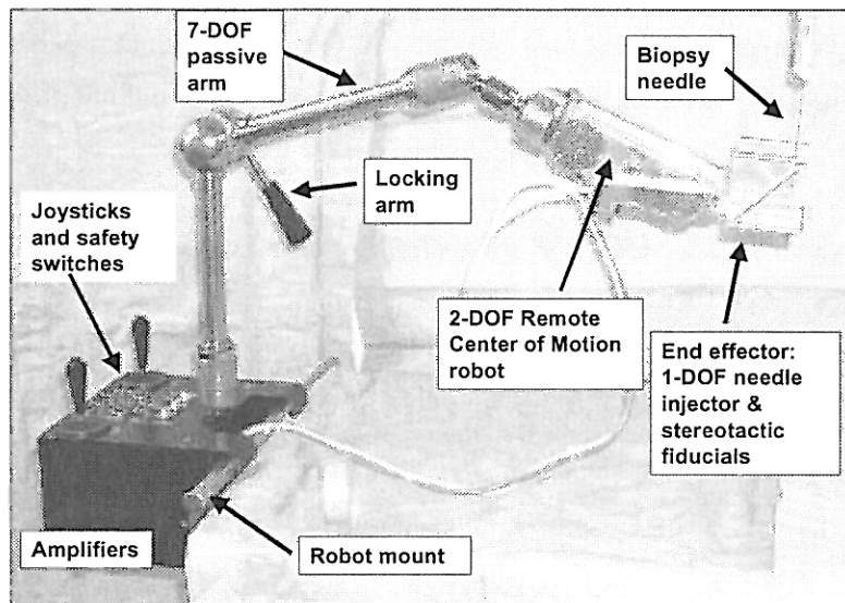
Figure 6: Pre-clinical prototype system
