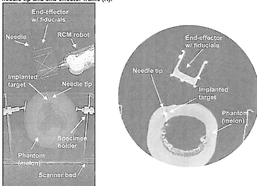
Figure 9: Confirmation images after needle insertion into the honeydew phantom. Scout view with target, needle, and robot (L). Image slice with implanted target, needle tip and end-effector frame (R).
