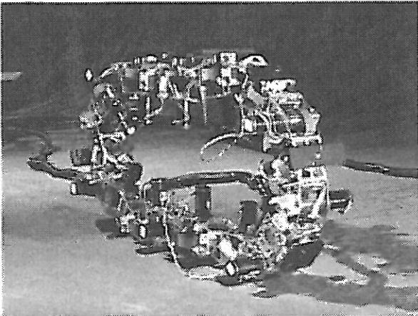
Figure 3: A loop of 23 G2 modules using rolling track locomotion.
