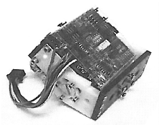
Figure 1: A G1v4 module with a communications cable attached. Two of four connection plates are visible. Two AAA batteries are mounted on the backside.
