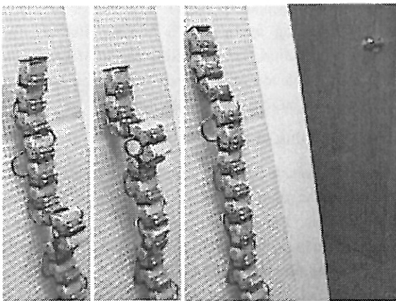
Figure 7: Caterpillar locomotion climbing a near vertical porous material (ceiling tile)
