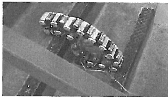
Figure 6: A loop configuration conforming to terrain as it climbs stairs,
