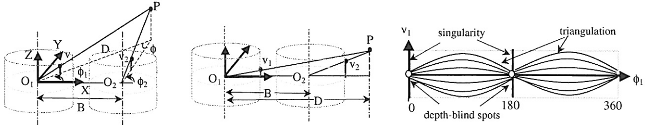
Fig. 1. Horizontally-aligned omnistereo (a) triangulation (b) singularity (2) epipolar curves
