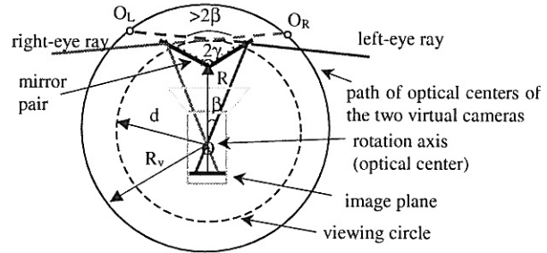
Fig. 6. A simple catadioptric approach
