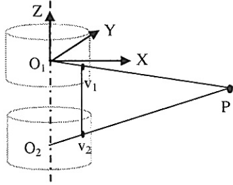
Fig. 2. Vertically-aligned omnistere
