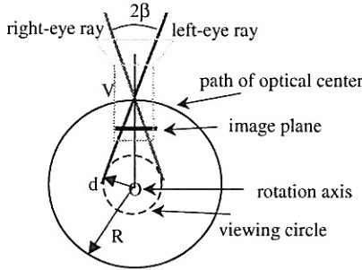
Fig. 5. A single-camera approach
