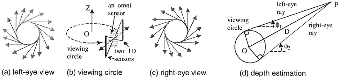
Fig. 4. Circular projection omnistere
