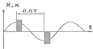
Figure 4. The one-way adjustment-motion strategy, where the sine-wave is the displacement of the DLO and the blocks are the acceleration and deceleration.
