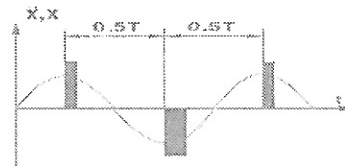
Figure 5. The two-way adjustment-motion strategy, where sine-line is the displacement of the DLO and blocks are the acceleration and deceleration.
