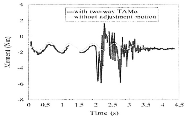
Figure 9. Measured moment M_y during the force/torque sensor-based adjustment-motion process
