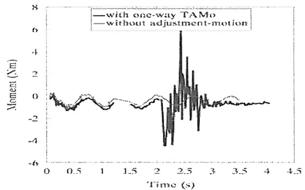
Figure 8. Measured moment M_y during the force/torque sensor-based adjustment-motion process
