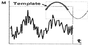
Figure 6. The template function: a half sine curve is used as the template and compared with the signal from sensor. The signal is drawn using raw data without smoothing.
