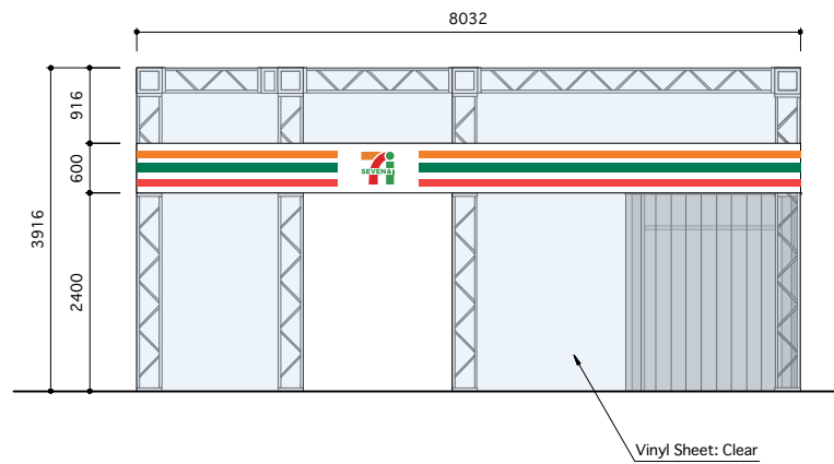
Elevation from point A (1:100)
