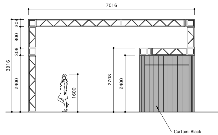
Elevation from point B (1:100)
